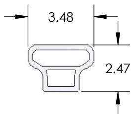
Railing
